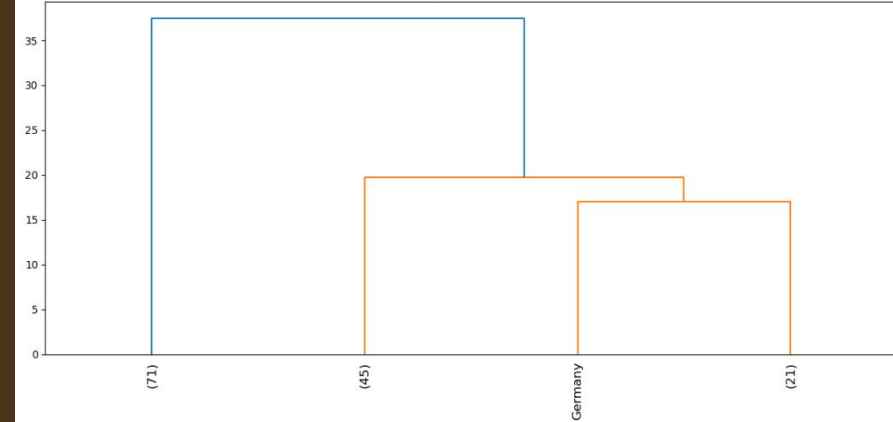
Dendrogramme (4 clusters)
