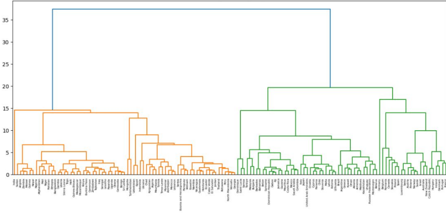
Dendrogramme (CAH)
